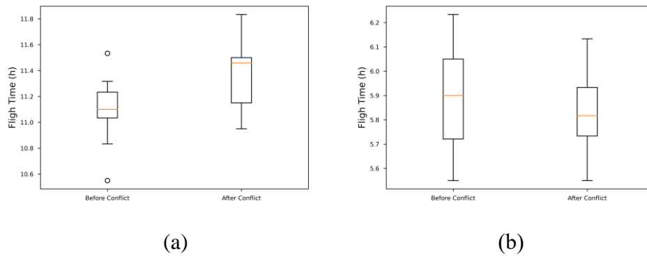
Figure 3. Boxplot of flight time records in before and after conflict datasets. (a) Paris, France to Tokyo, Japan ( p=0.0016689 ). (b) Beijing, China to Singapore ( p=0.76825 ).
