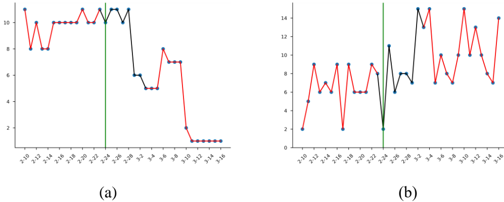
Figure 5. Variation of flight number in two typical airlines
