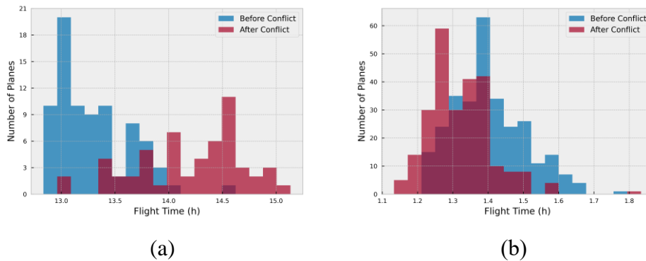
Figure 4. Histograms of flight time between an OD airport. (a) Toronto, Canada to Incheon South Korea ( p=2.6488e-17 ). (b) Geneva, Switzerland to London, the UK ( p=1.0 ).
